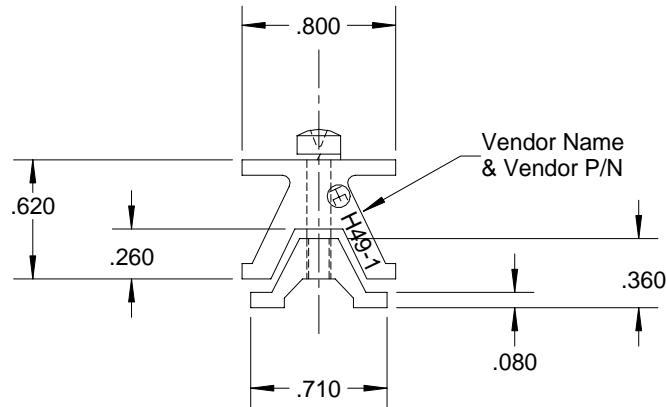
-1 END CLAMP ASSY (SHOWN) -2 & -3 END CLAMP ASSY (AS NOTED)
