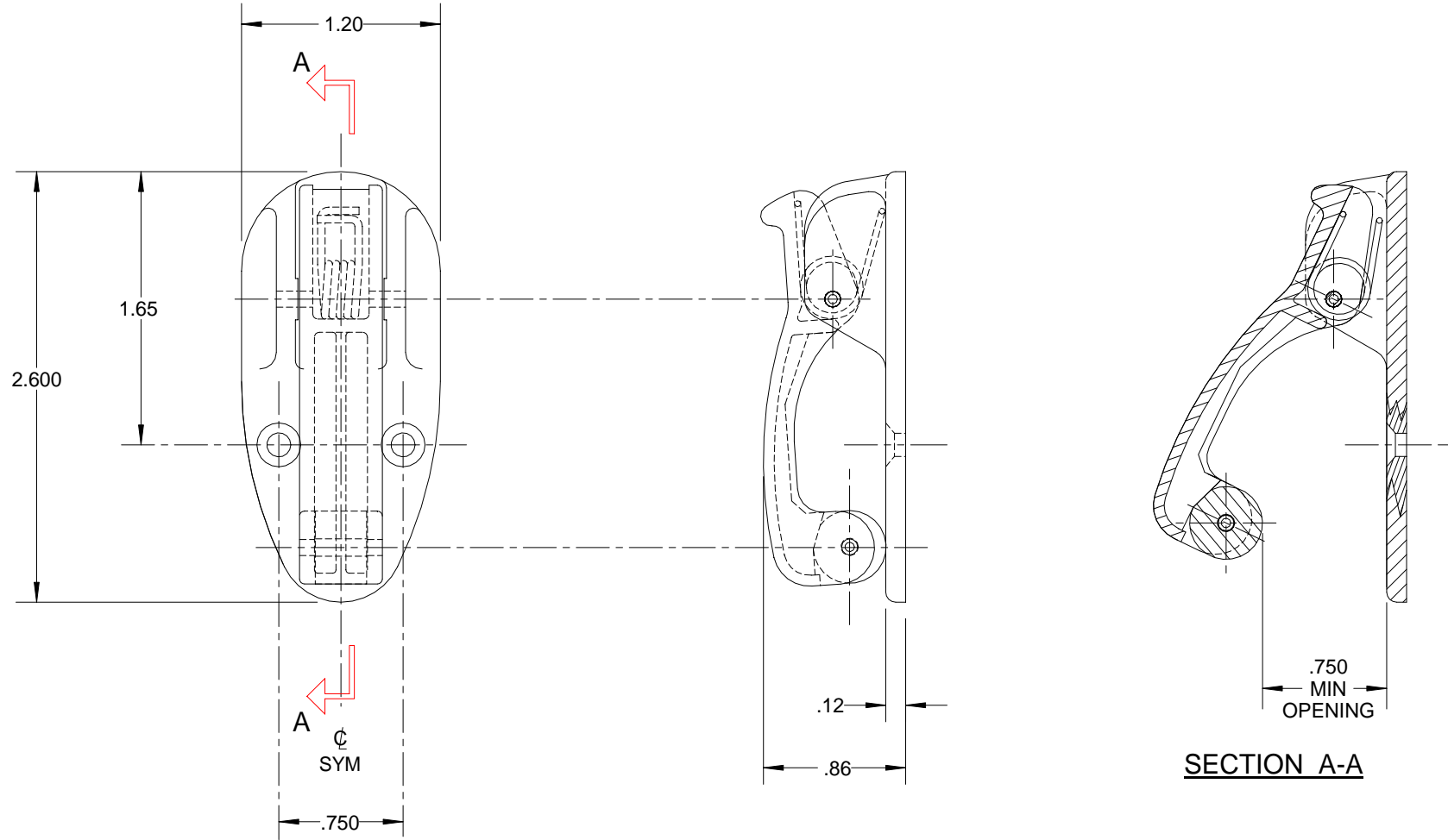
-1(X) ASSY
