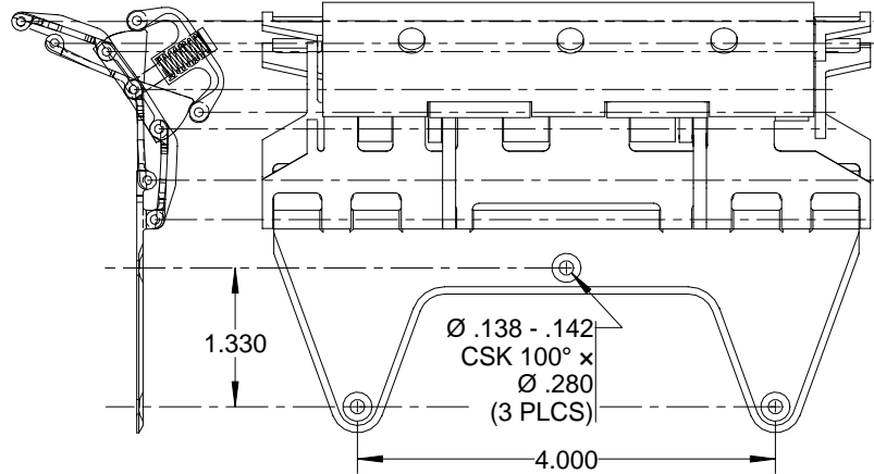
-1 HINGE ASSY
