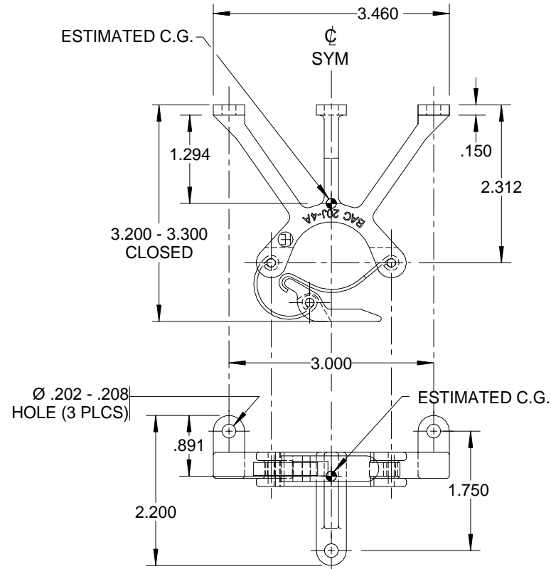
-1 BRACKET ASSEMBLY
