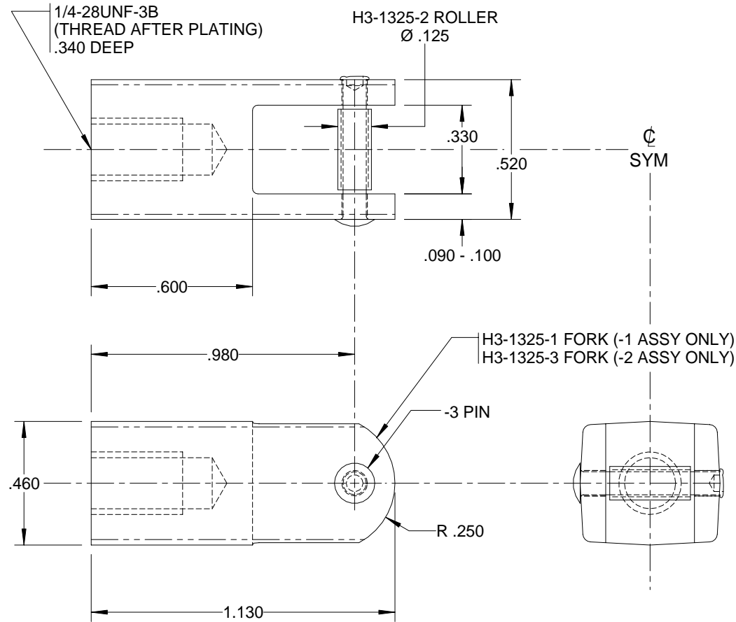
-1 FORK ASSY (Chrome) -2 FORK ASSY (Black) 2X SIZE
