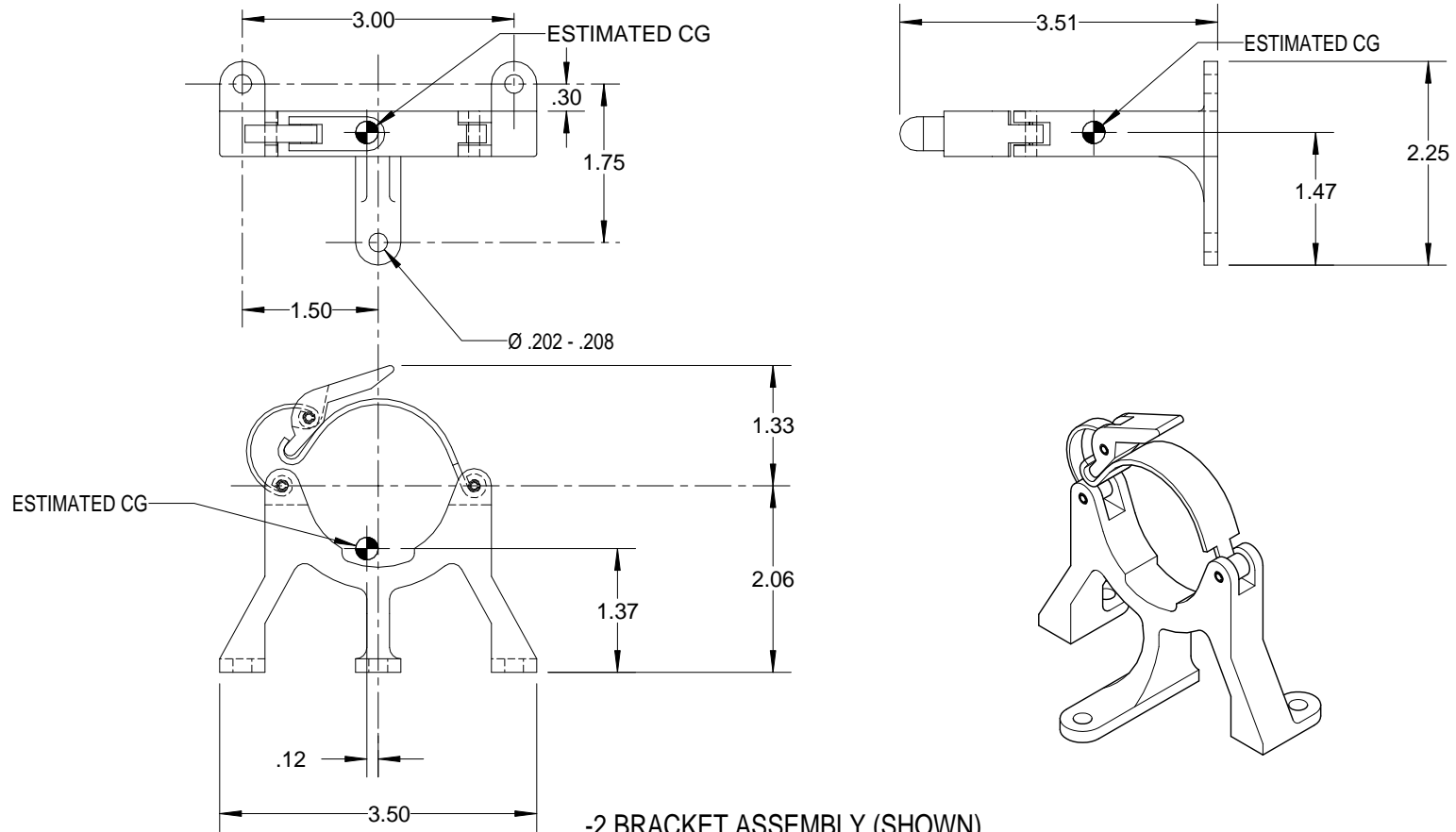
-2 BRACKET ASSEMBLY (SHOWN) -3 BRACKET ASSEMBLY (OPPOSITE -2)
