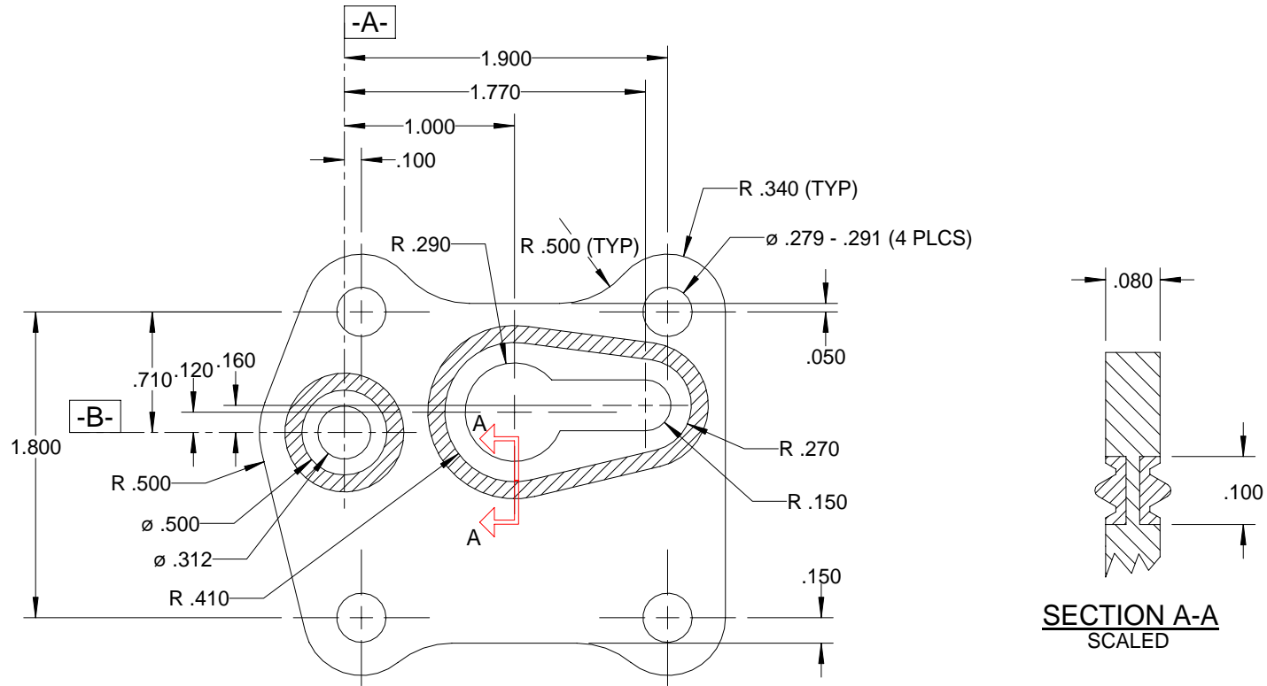
H3-1137 SEAL PLATE
