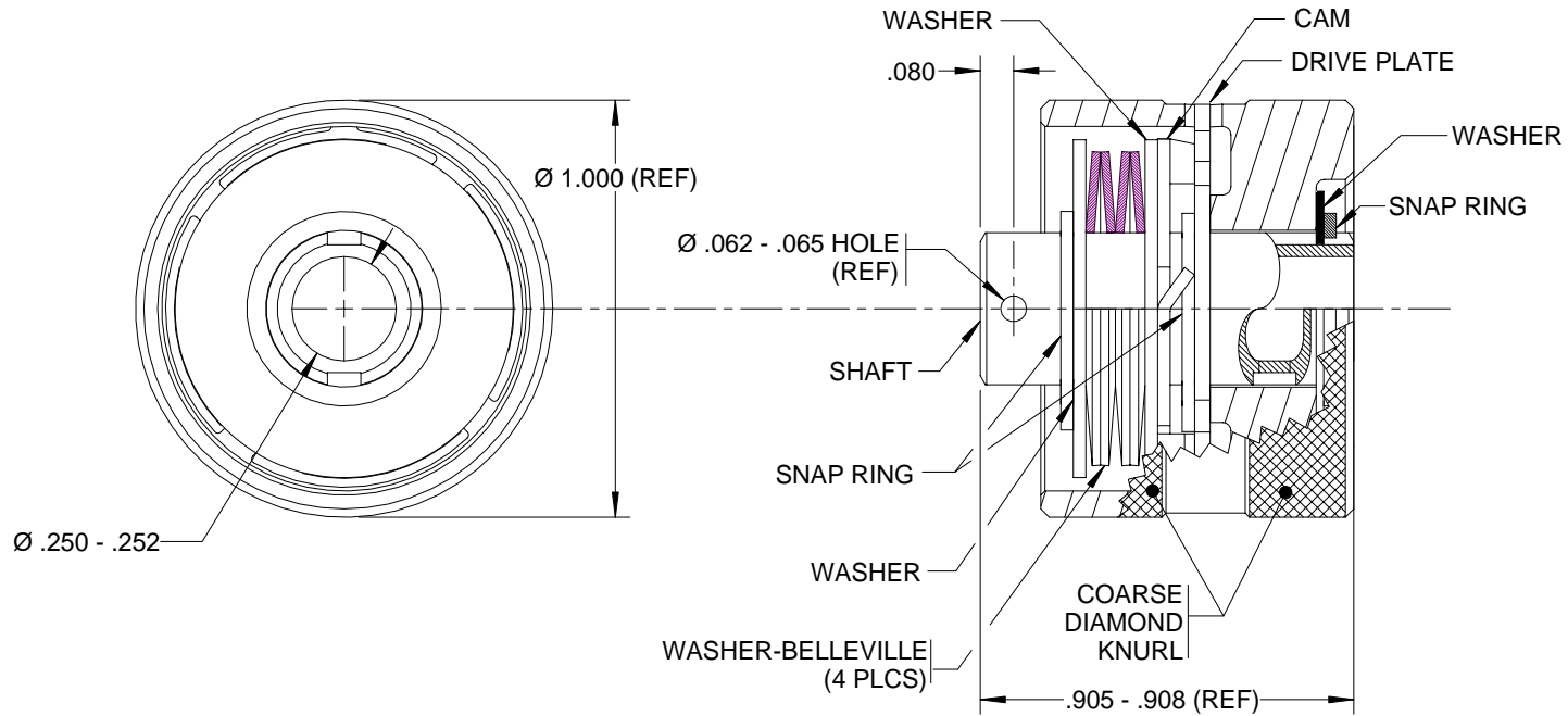
-1 KNOB ASSY
