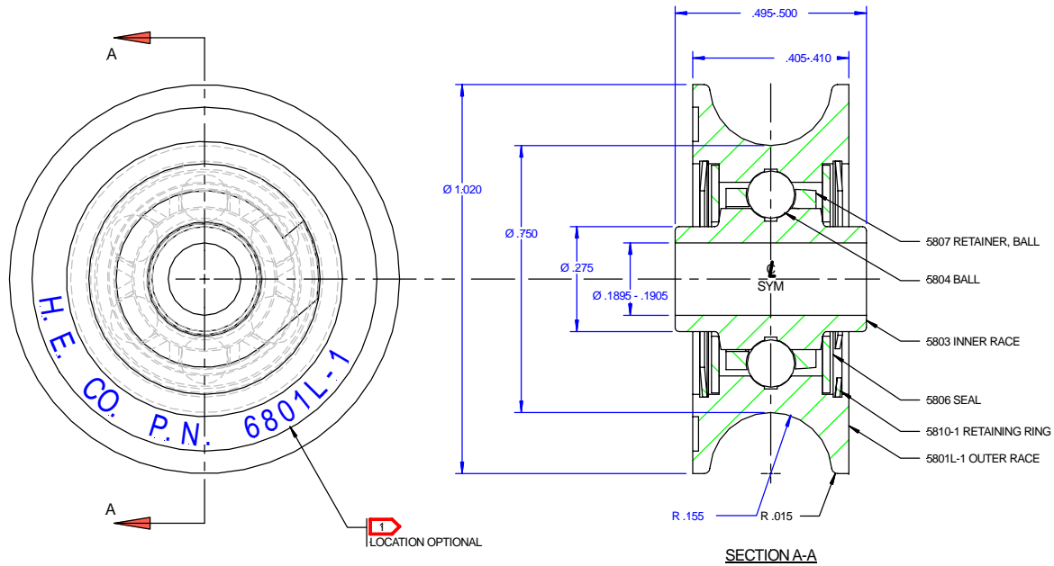
6801L-1 PULLEY ASSY SCALE 4:1
